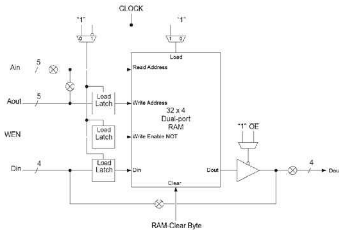
Figure 7-2. RAM logic - Detailed
