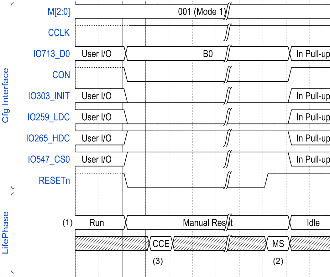
Figure 5-9. ATF280F: Manual Reset in mode 1
