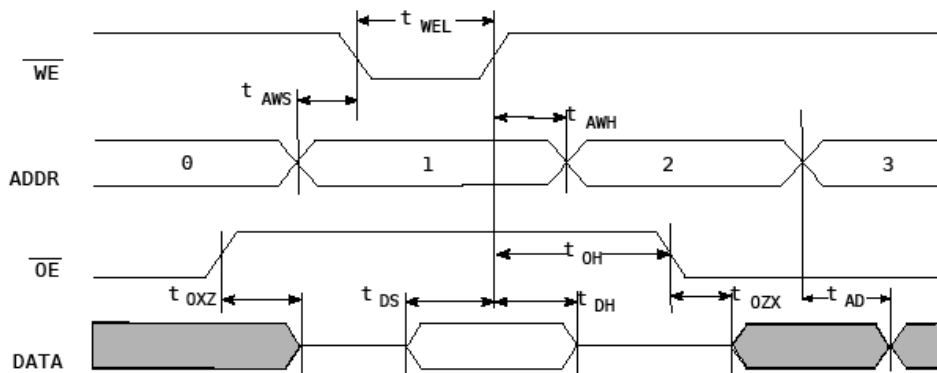
Figure 16-3. Single-port Write/Read
