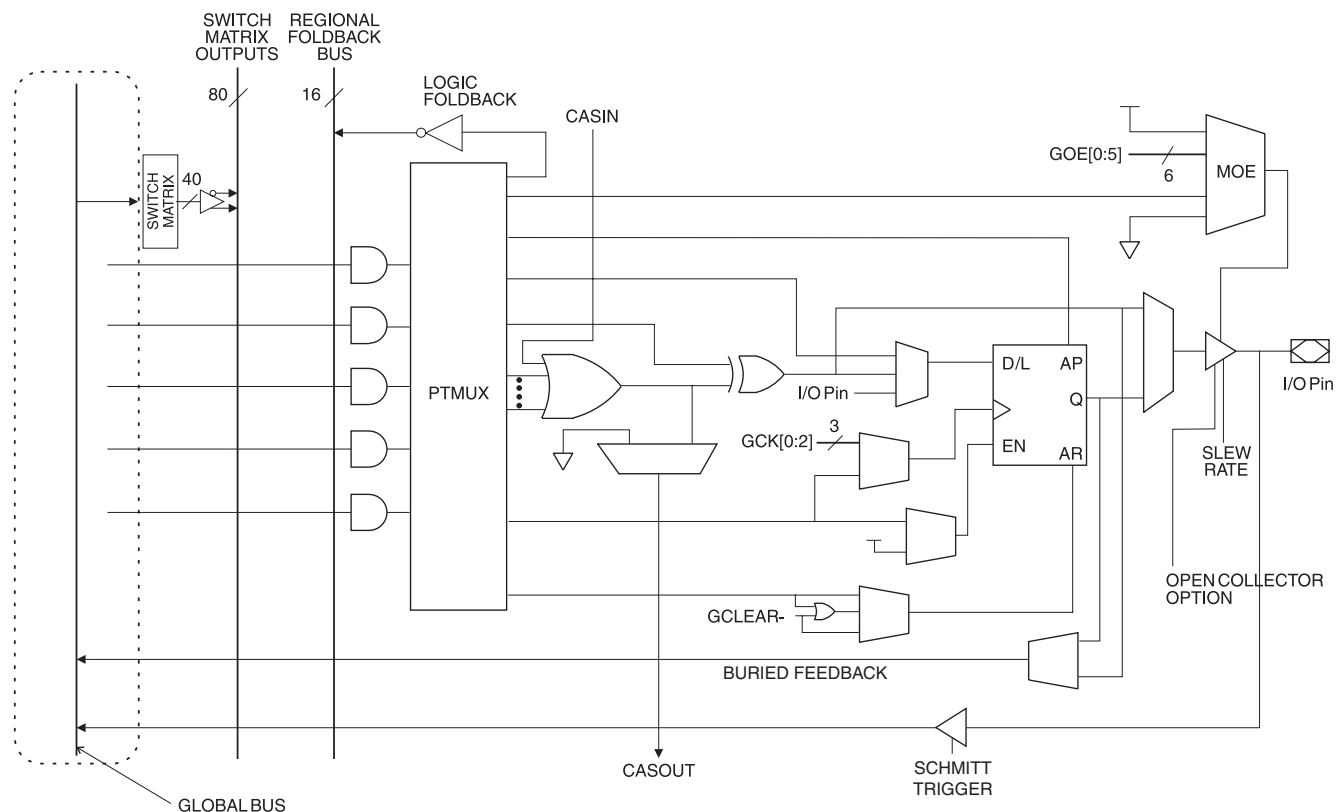
Figure 1-3. ATF1502BE Macrocell
