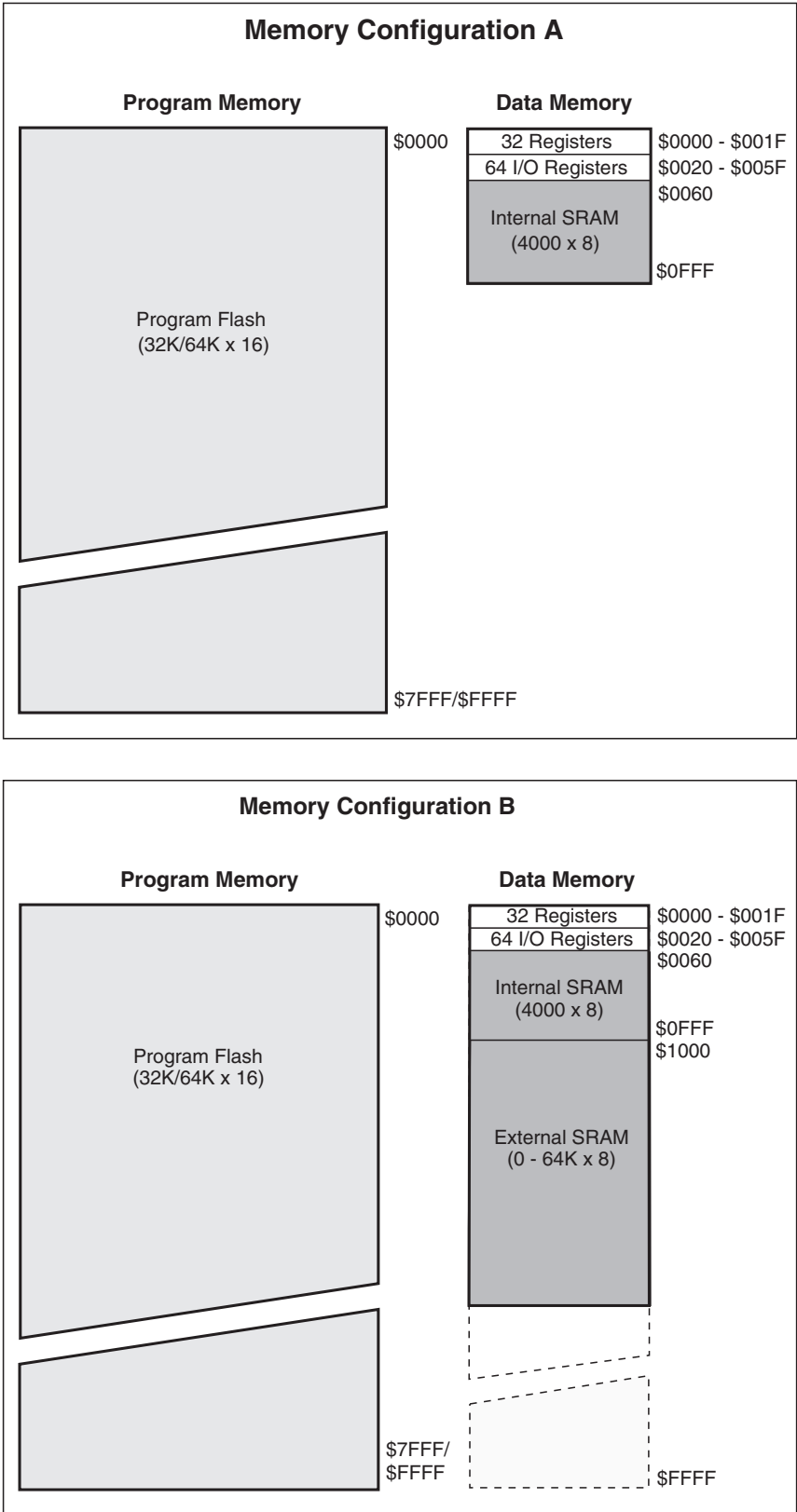
Figure 7. Memory Configurations
