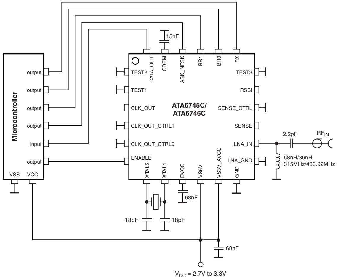
Figure 9-1. 3V Application
