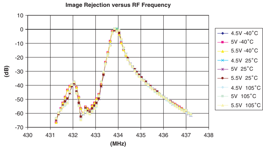
Figure 5-1. Narrow Band Receiving Frequency Response Atmel ATA5724C
