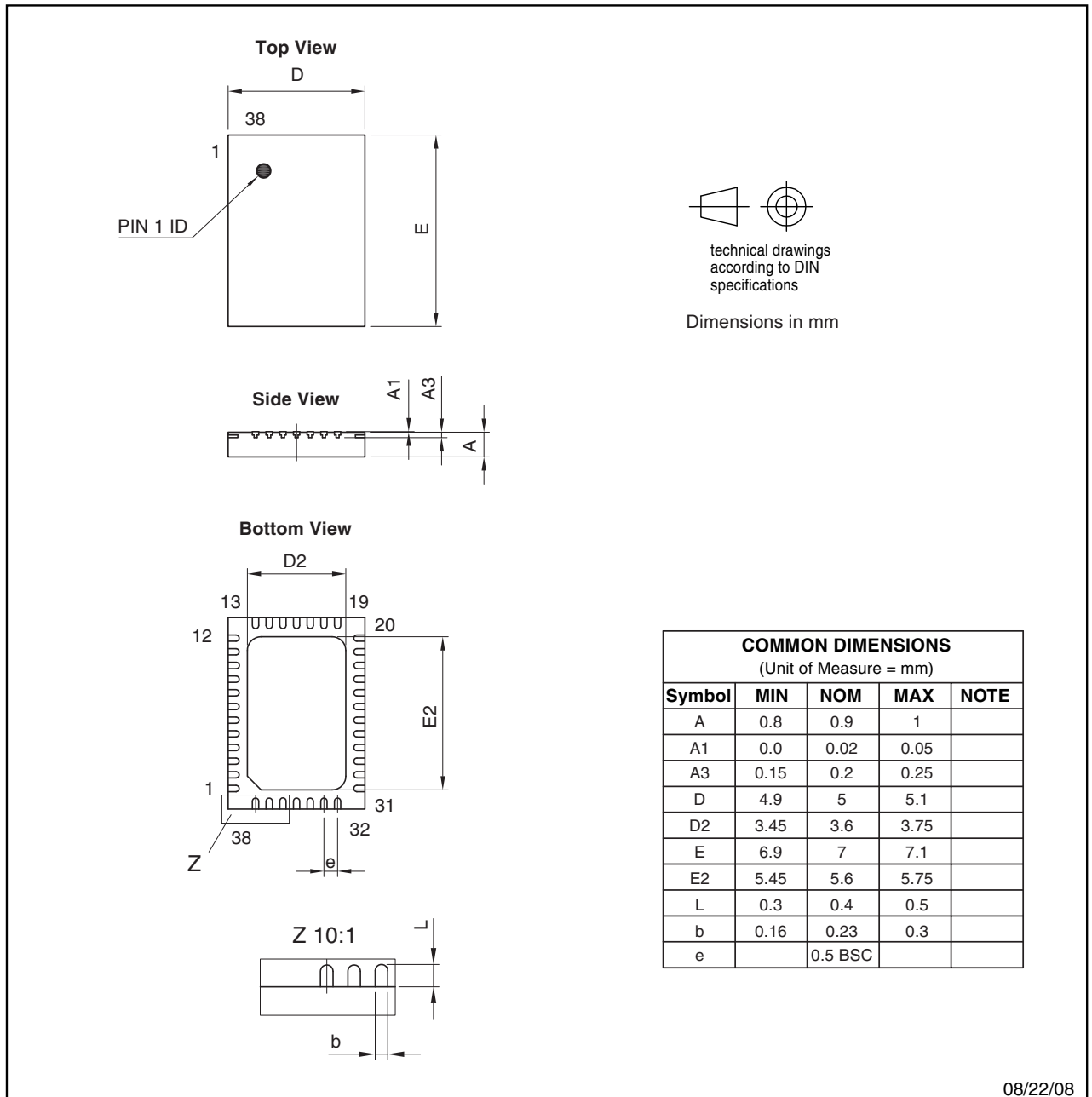
Figure 3-1. QFN 38 - 5x7 Package
