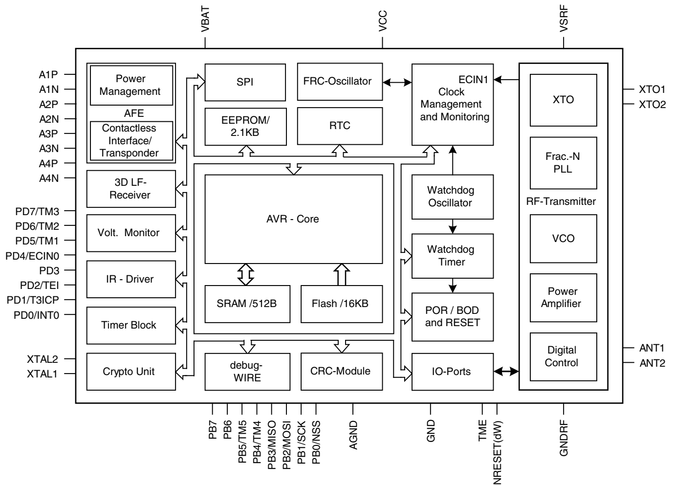
Figure 1-2. Atmel® ATA5791 Block Diagram
