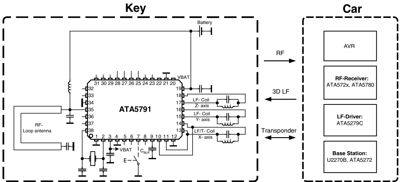
Figure 1-1. System Block Diagram
