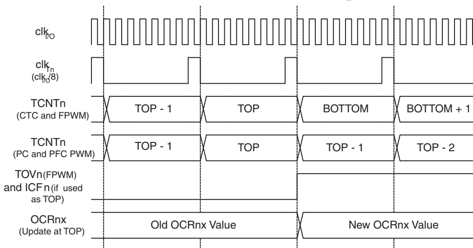
Figure 4-49. Timer/Counter Timing Diagram, with Prescaler ( f_{\text{clk\_I/O}}/8 )
