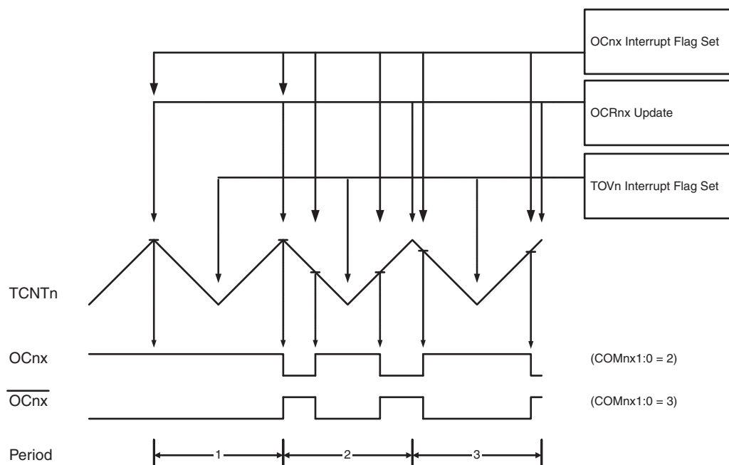
Figure 4-36. Phase Correct PWM Mode, Timing Diagram
