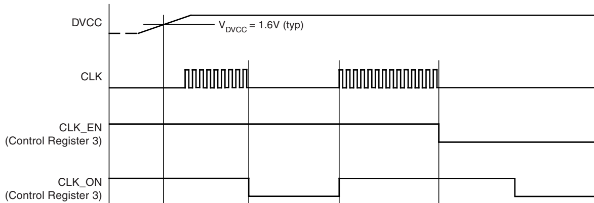
Figure 9-3. Clock Timing
