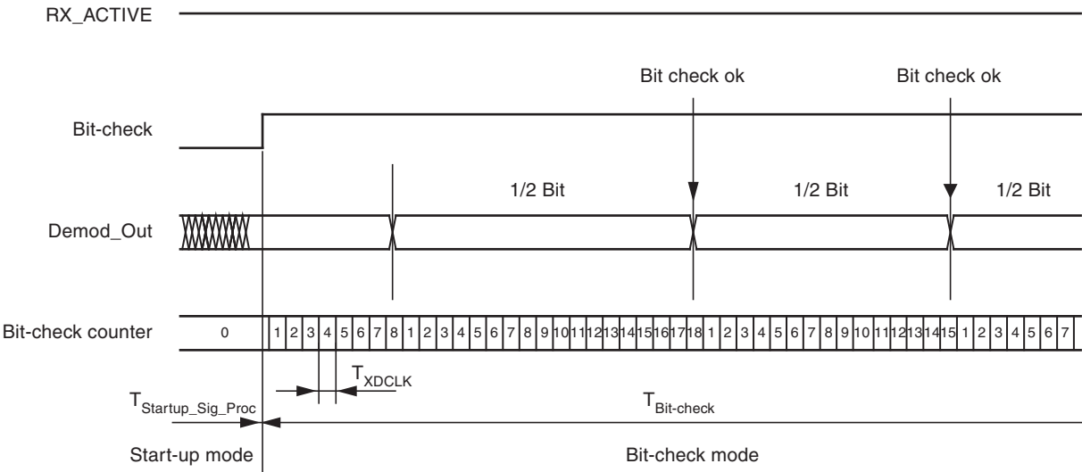
Figure 14-4. Timing Diagram During Bit-check (Lim_min = 14, Lim_max = 24)
