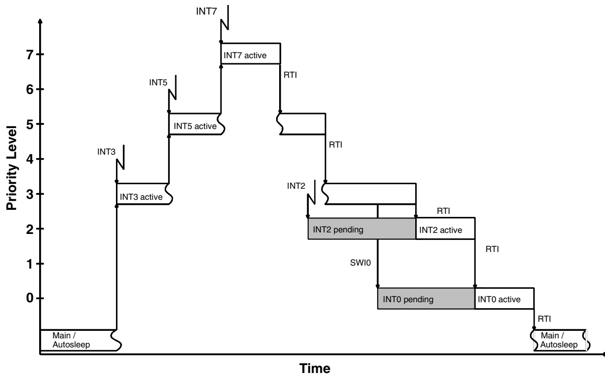
Figure 4-6. Interrupt Handling
