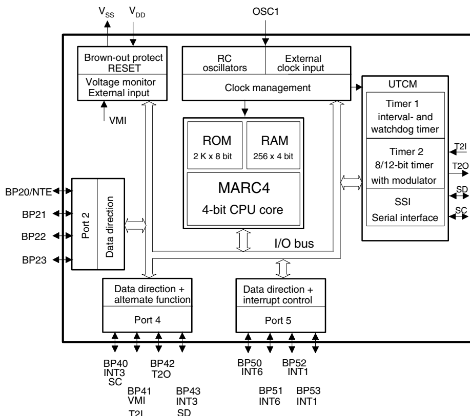
Figure 1-1. Block Diagram
