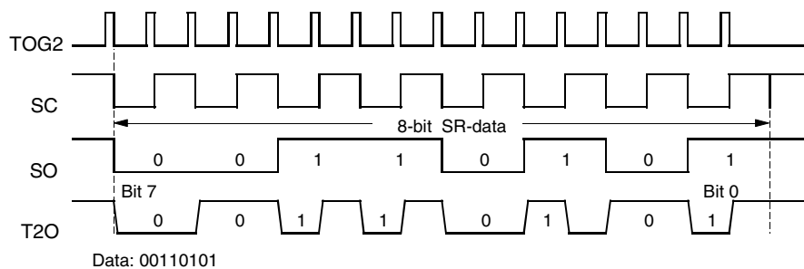
Figure 5-34. Bi-phase Modulation 1
