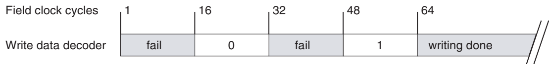
Figure 9-1. Write Data Decoding Scheme
