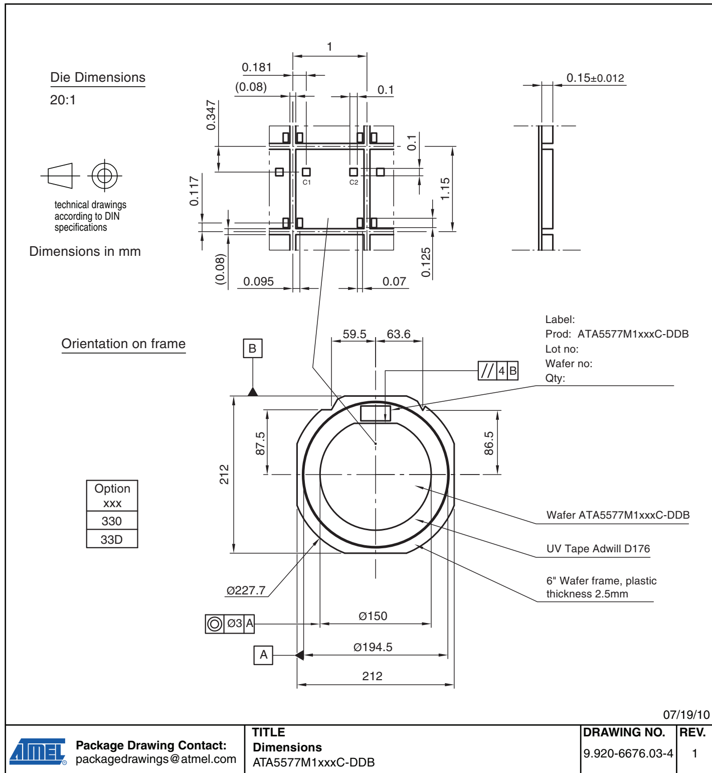
Figure 11-1. Sawn Wafer on Foil with Ring (Type 1, Standard Pads)
