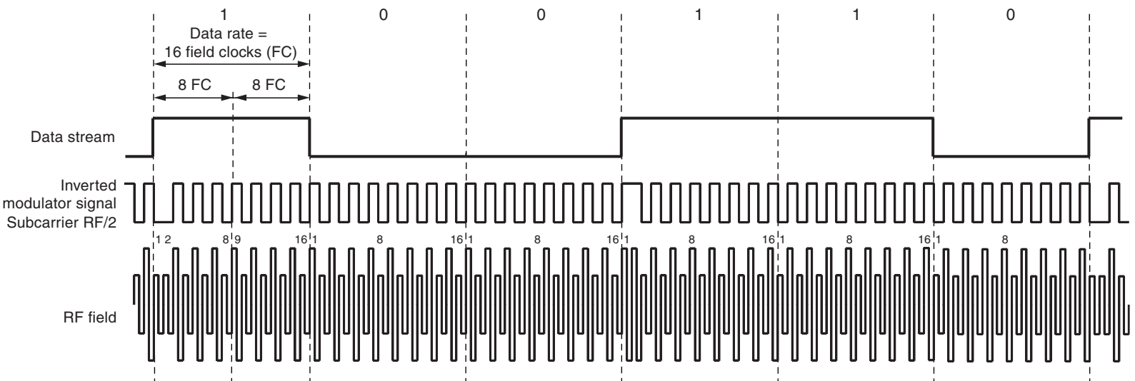
Figure 6-7. Example of PSK3 Coding with Data Rate RF/16
