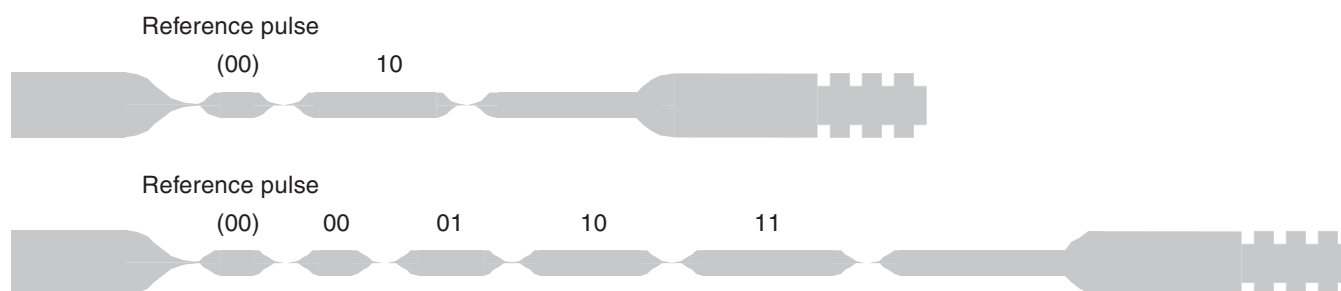
Figure 5-15. 1-of-4-coding Protocol
