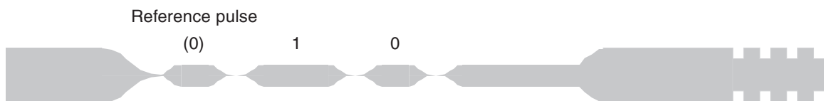
Figure 5-14. Leading-zero-reference Protocol
