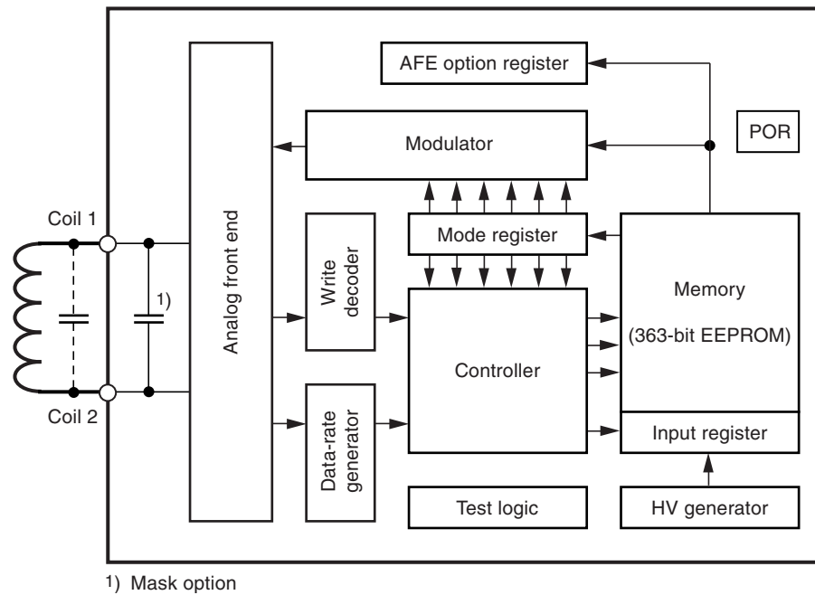
Figure 4-1. Block Diagram
