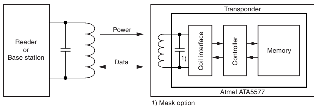
Figure 3-1. RFID System Using Atmel ATA5577C Tag
