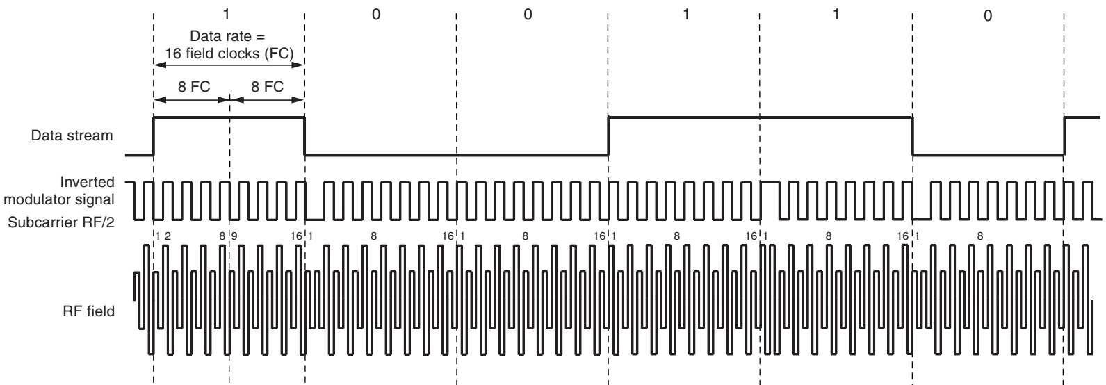
Figure 6-6. Example of PSK2 Coding with Data Rate RF/16
