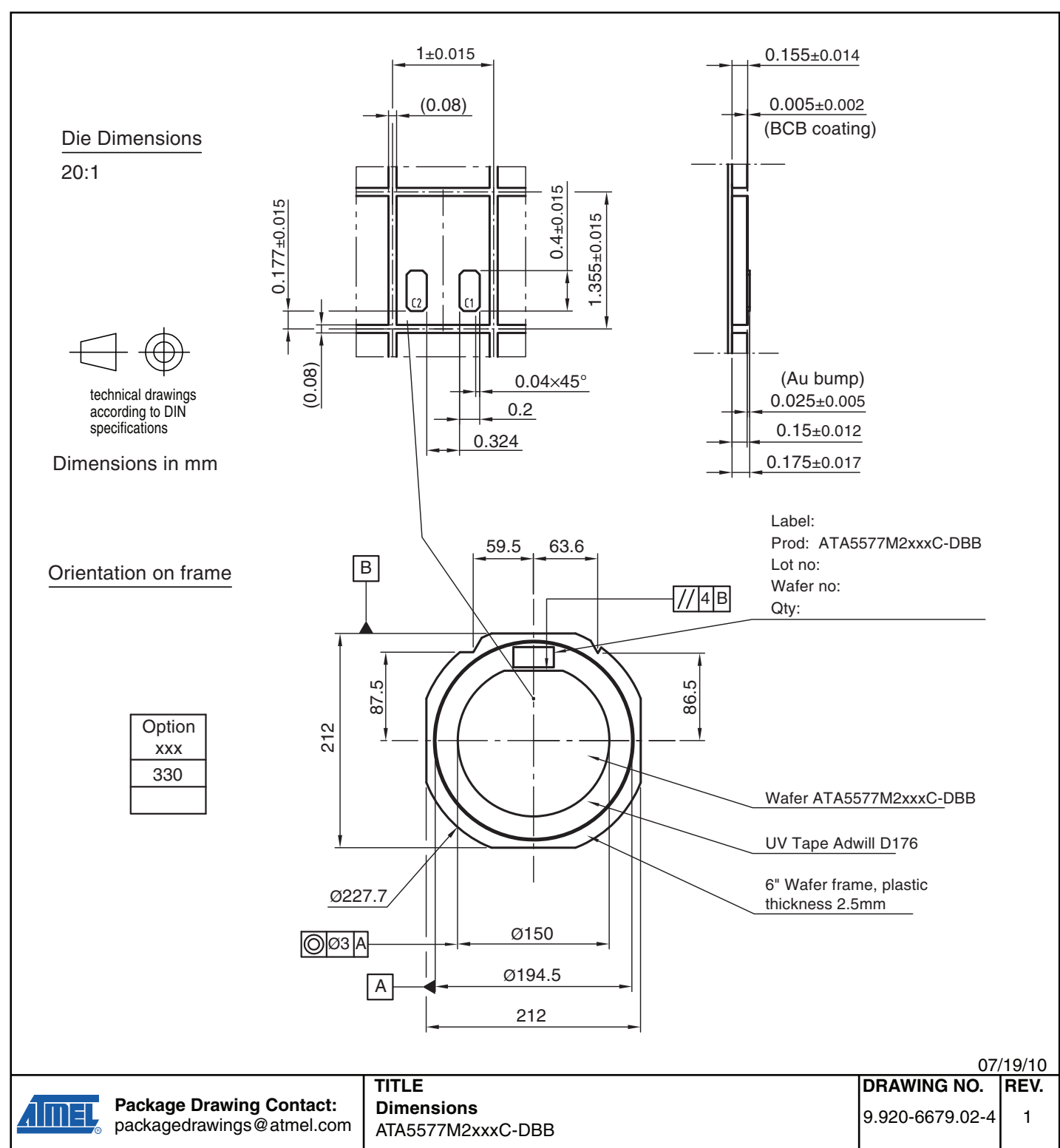
Figure 11-3. Sawn Wafer on Foil with Ring (Type 2, Mega Pads and Au Bumps)
