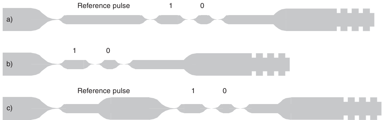
Figure 5-13. Long-leading-reference Protocol
