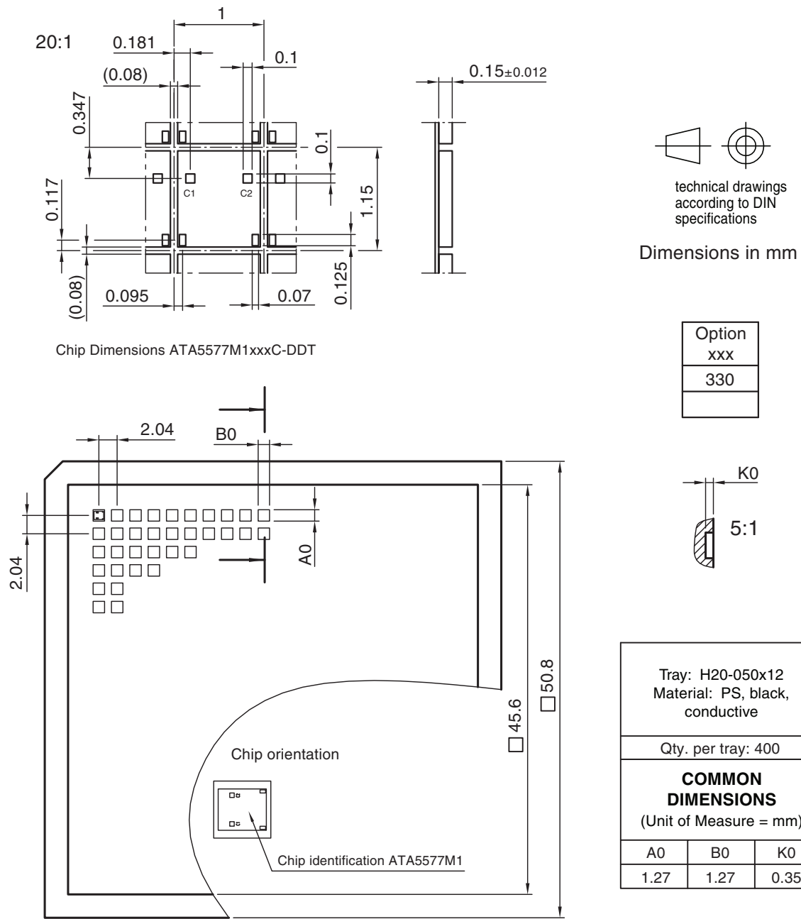
Figure 11-2. Die in Waffle Pack
