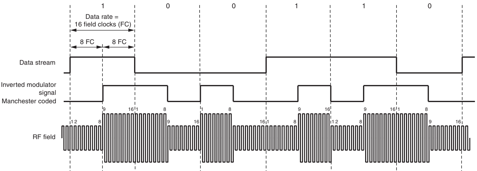
Figure 6-2. Example with Manchester Coding with Data Rate RF/16
