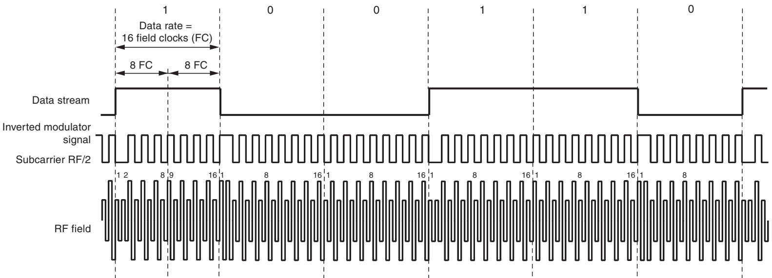
Figure 6-5. Example of PSK1 Coding with Data Rate RF/16
