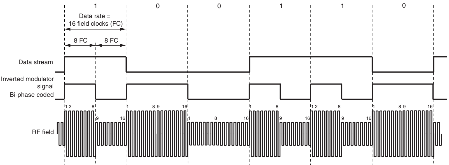
Figure 6-3. Example of Bi-phase Coding with Data Rate RF/16
