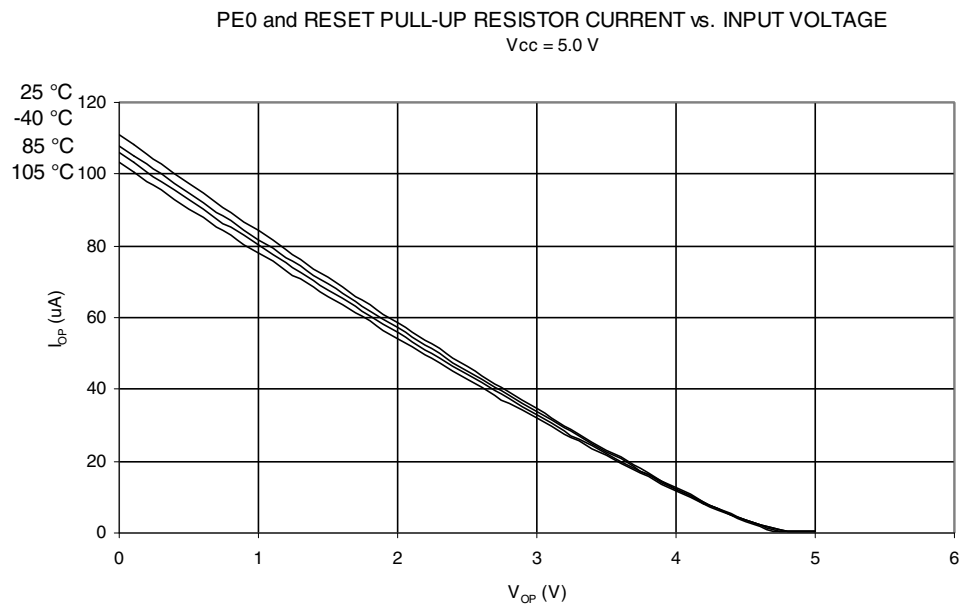
Figure 27-14. Reset Pull-Up Resistor Current vs. Reset Pin Voltage ( V_{CC} = 5V )
