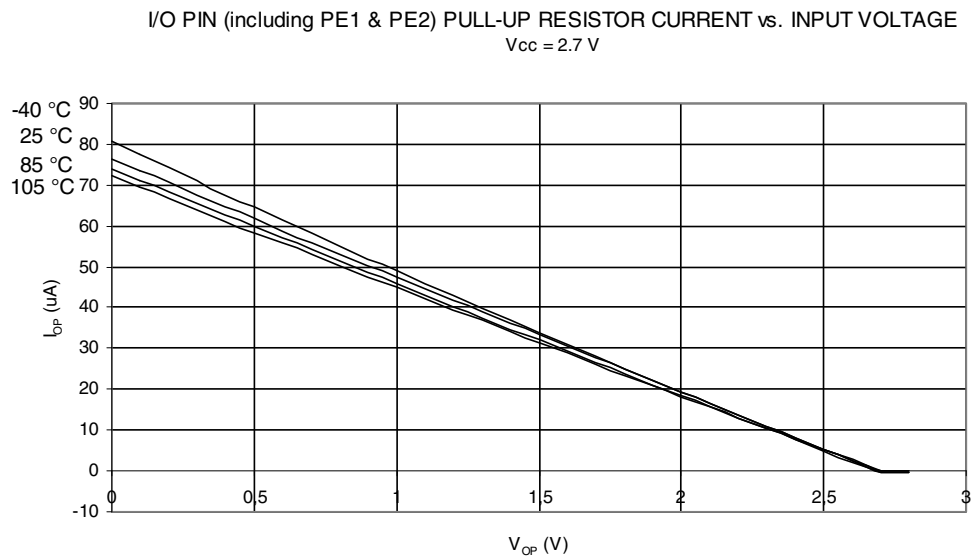
Figure 27-13. I/O Pin Pull-Up Resistor Current vs. Input Voltage ( V_{CC} = 2.7V )
