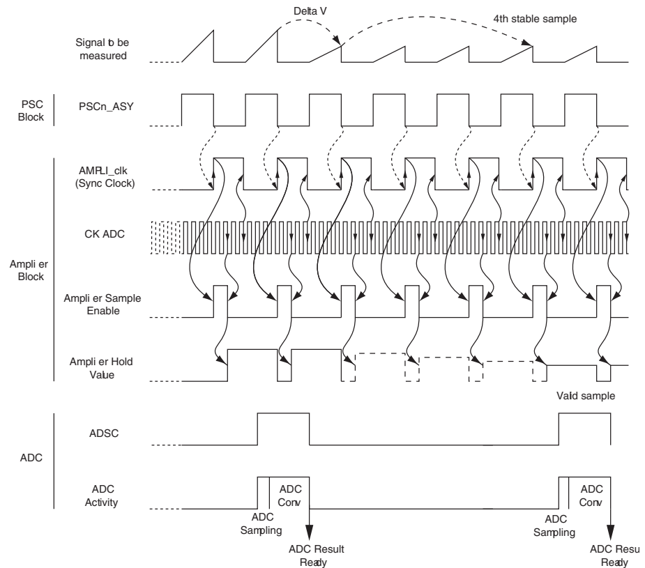
Figure 21-15. Amplifier synchronization timing diagram with change on analog input signal.
