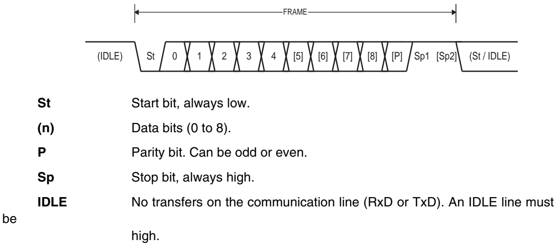
Figure 18-4. Frame Formats
