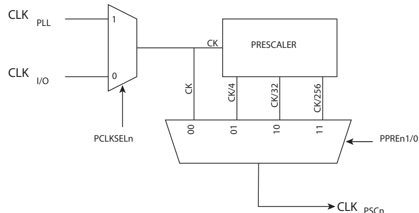
Figure 16-39. Clock selection
