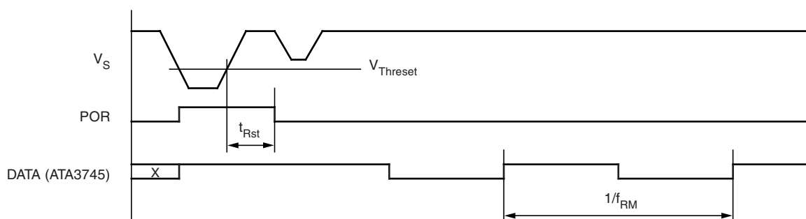
Figure 5-13. Generation of the Power-on Reset
