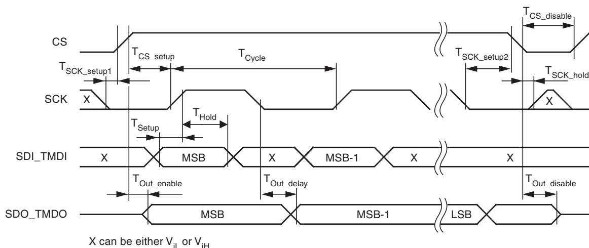
Figure 8-7. Serial Timing
