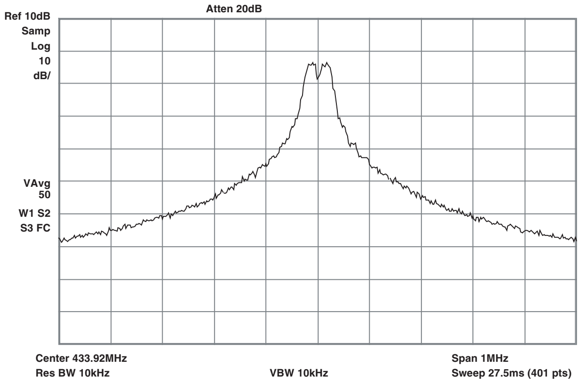
Figure 3-9. FSK-modulated TX Spectrum (433.92MHz/20Kbit/s/ \pm 16.17 kHz/Manchester Code)
