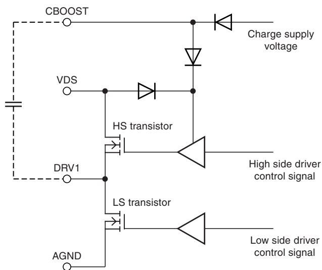
Figure 3-12. Bootstrap Configuration Circuitry
