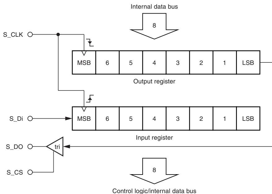
Figure 3-6. SPI Structure
