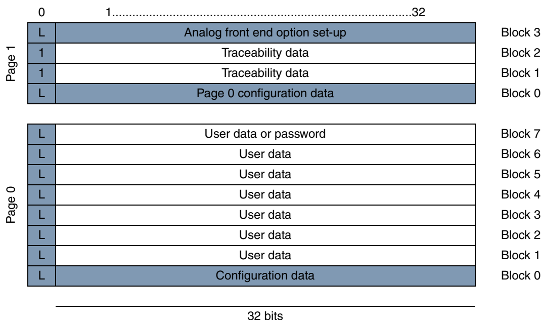
Figure 4-2. Memory Map
