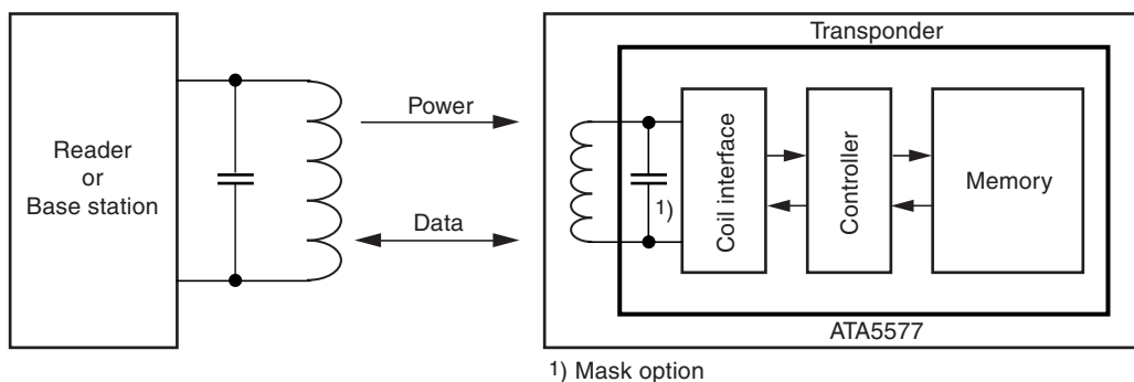
Figure 3-1. RFID System Using ATA5577 Tag
