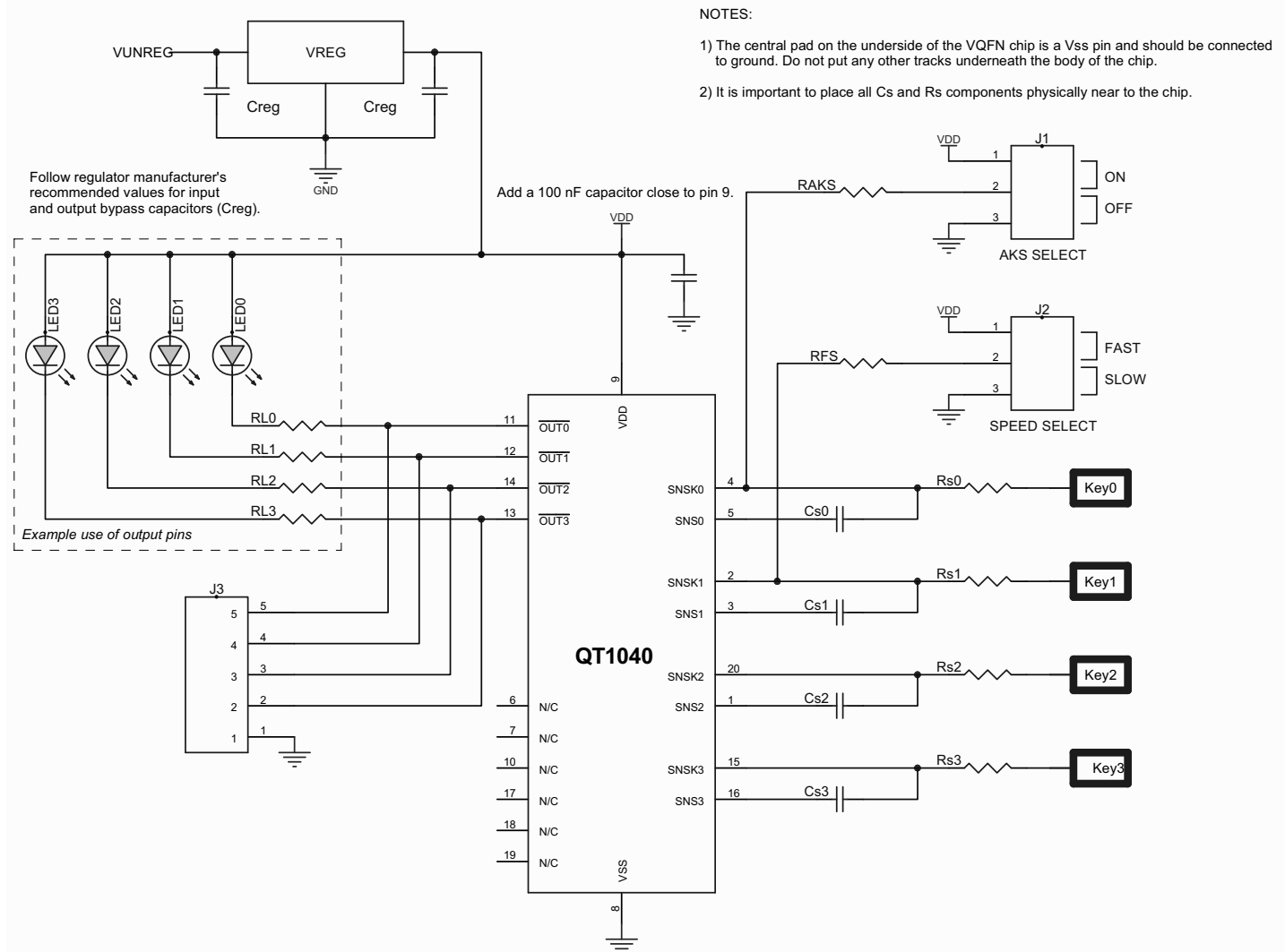
Figure 1-1. Typical Circuit
