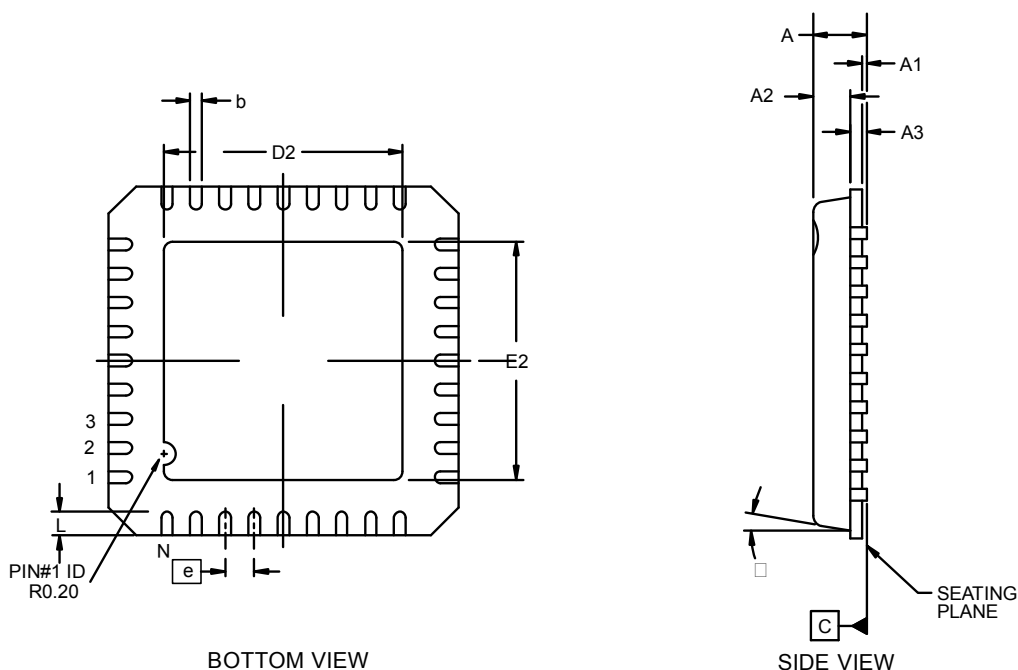
Figure D-1. AT88RF1354 6x6 mm QFN package
