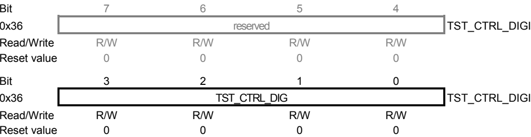
Figure 0-1. Register TST_CTRL_DIGI.
