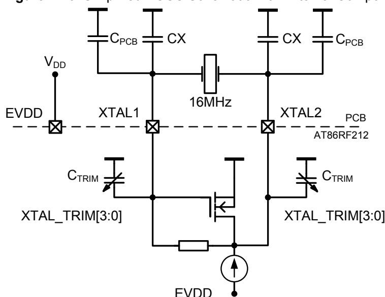
Figure 7-15. Simplified XOSC Schematic with External Components
