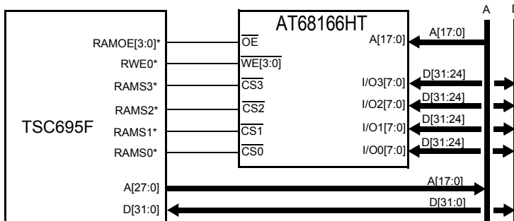
Figure 7. 8-bit typical application (four SRAM banks)
