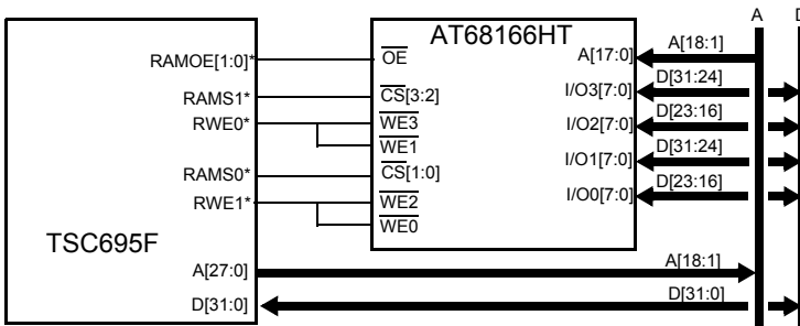
Figure 6. 16-bit typical application (two SRAM banks)
