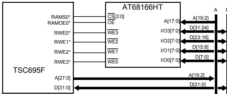
Figure 5. 32-bit typical application (one SRAM bank)
