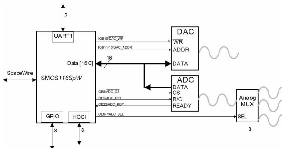
Figure 8-2. ADC/DAC Interface
