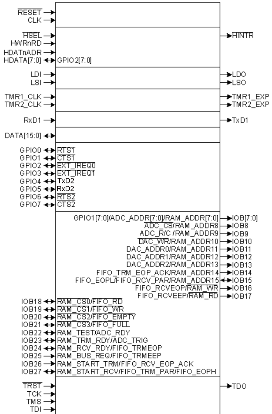
Figure 3-1. Signals Organization
