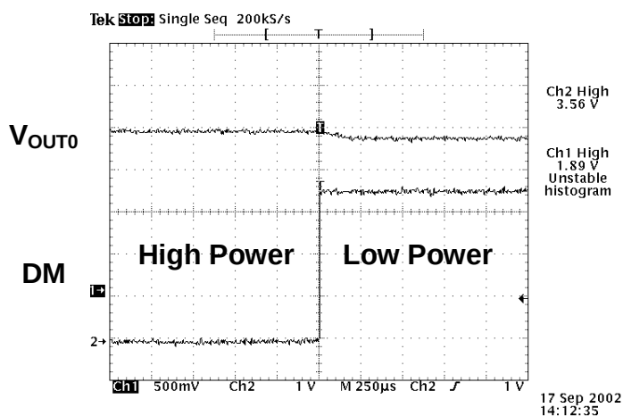
Figure 5. Low-power/Full-power DC-to-DC Converter Transition
