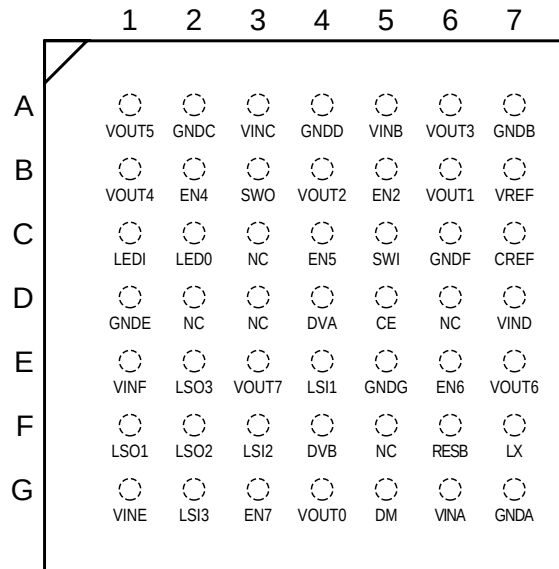
Figure 2. AT73C204 Pin Configuration in 49-ball BGA Package
