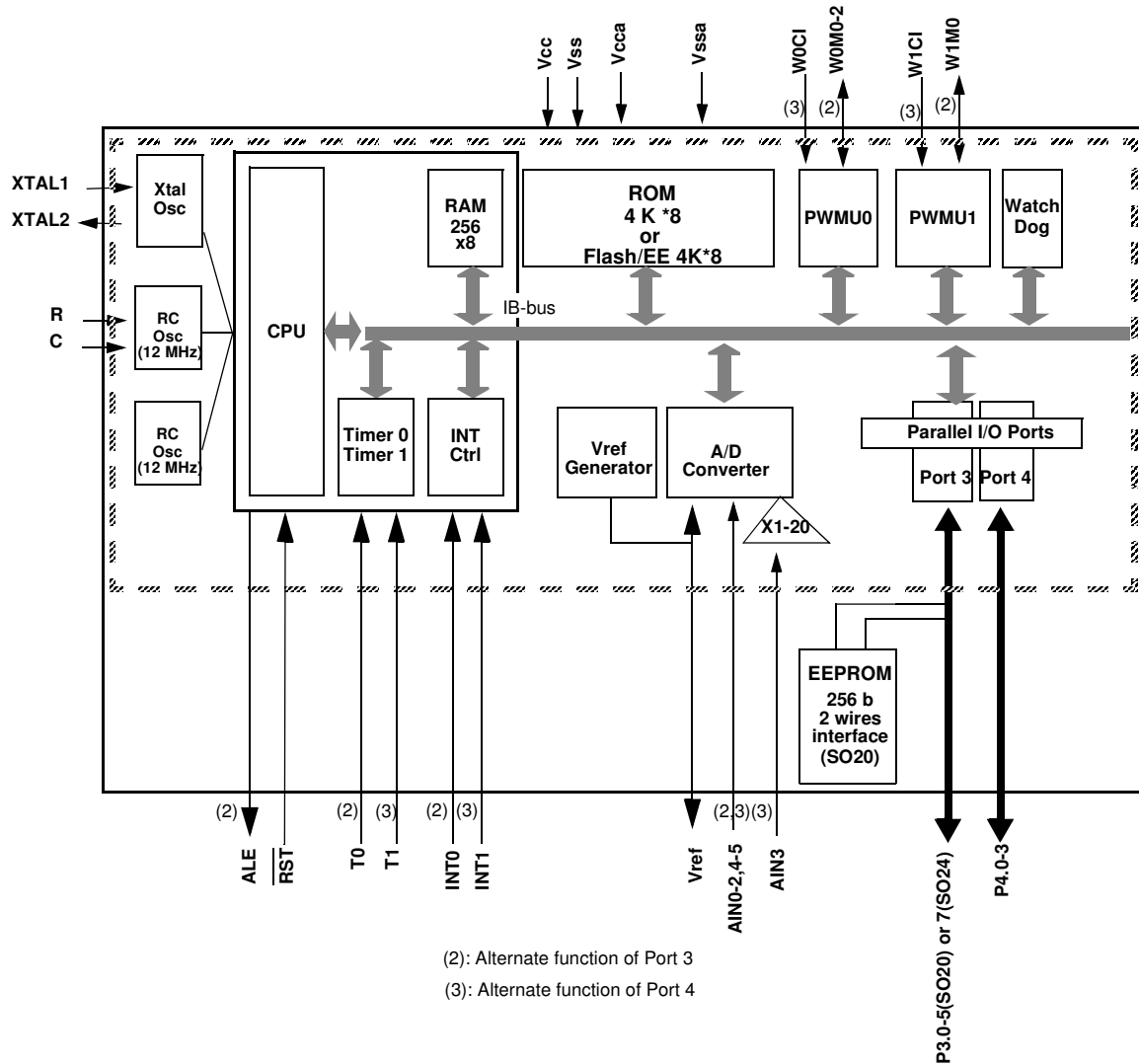
Figure 1. Block Diagram
