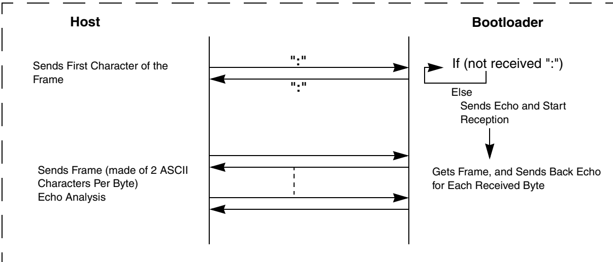
Figure 24-12. Command Flow
