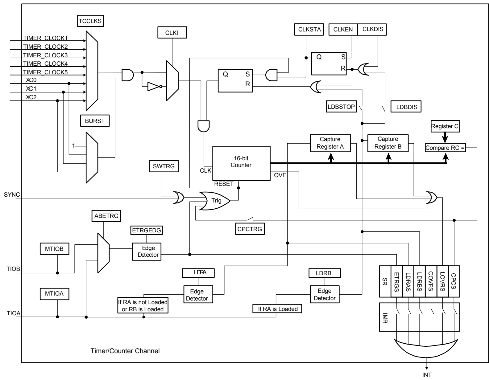
Figure 23-4. Capture Mode
