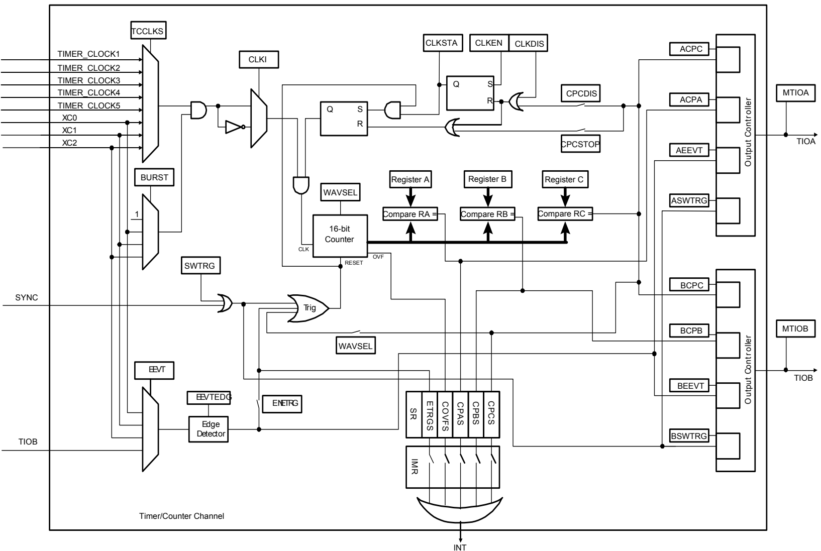
Figure 23-5. Waveform Mode
