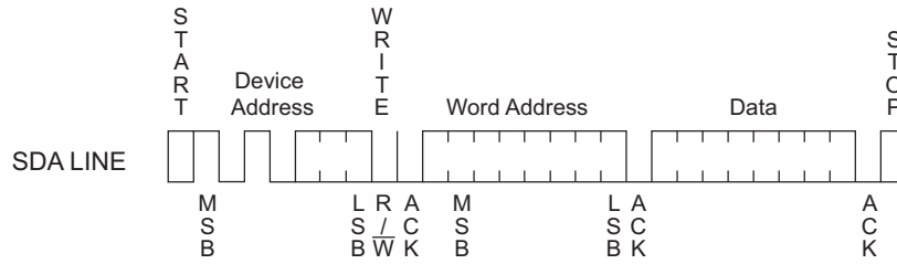
Figure 8-2. Byte Write
