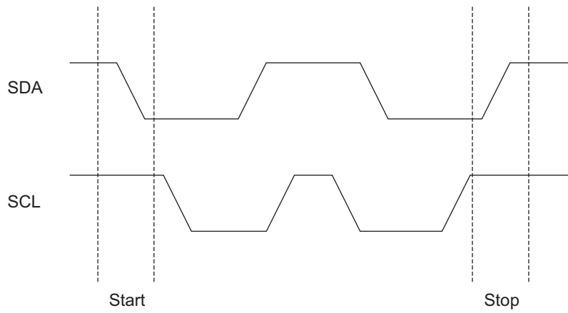
Figure 4-5. Start and Stop Condition
