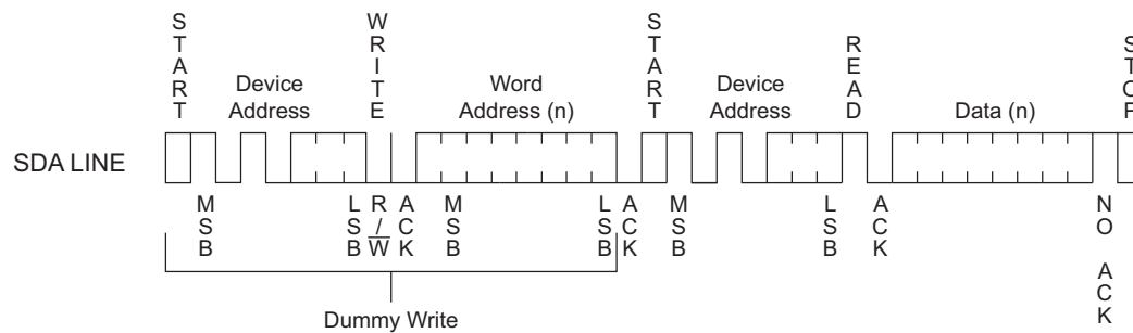
Figure 8-5. Random Read
