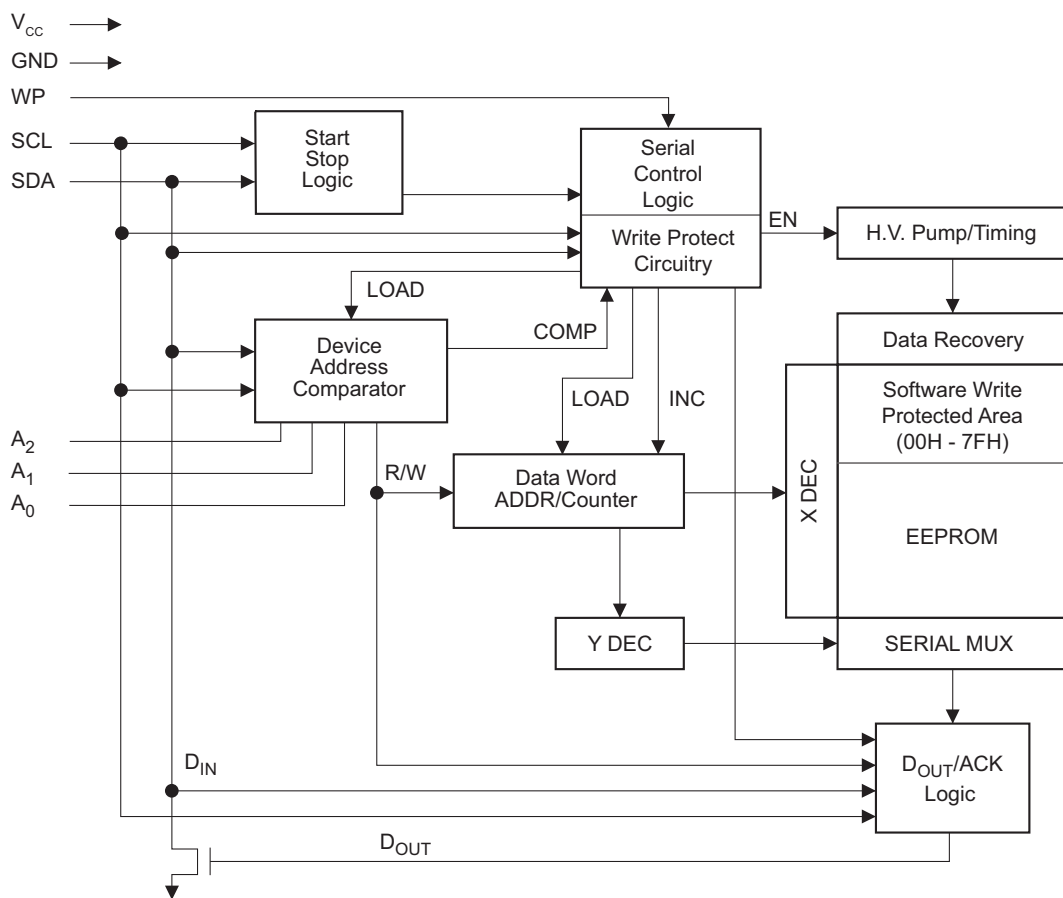
Figure 1-1. Block Diagram
