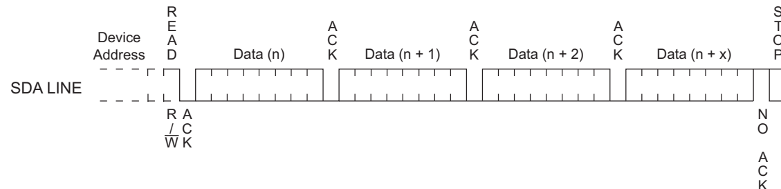
Figure 8-6. Sequential Read
