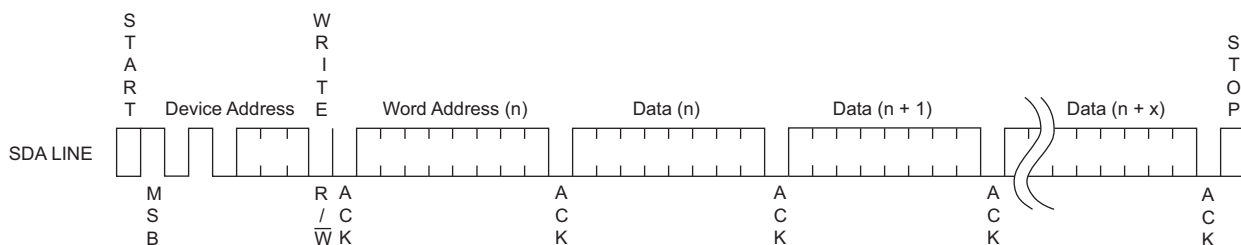
Figure 10-3. Page Write
