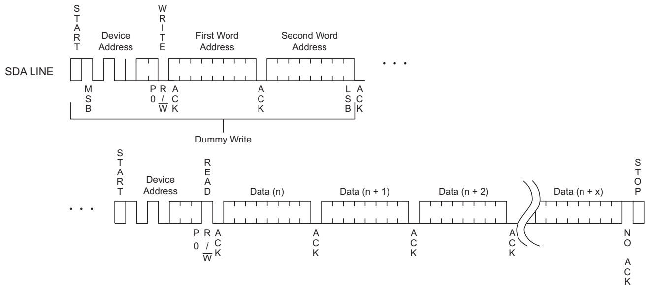
Figure 9-5. Sequential Read
