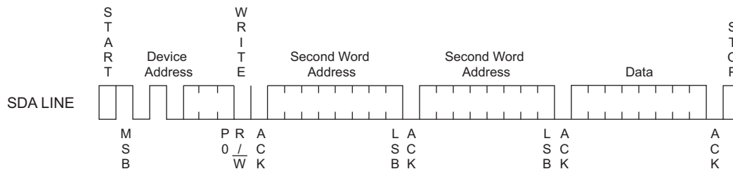
Figure 9-1. Byte Write
