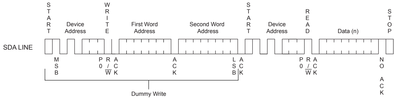
Figure 9-4. Random Read
