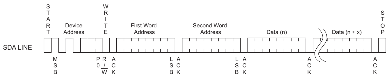
Figure 9-2. Page Write
