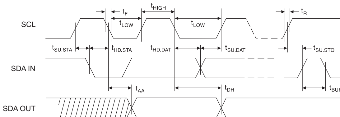
Figure 4-2. Bus Timing
