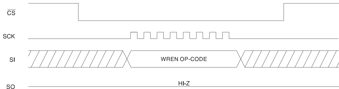
Figure 6-3. WRDI Timing
