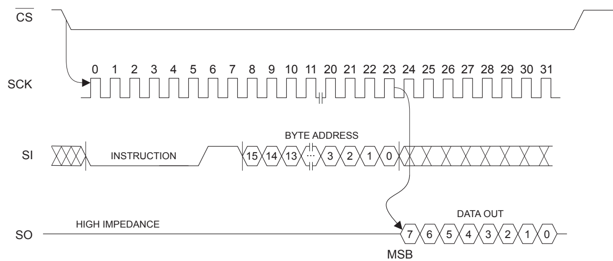
Figure 6-6. Read Timing
