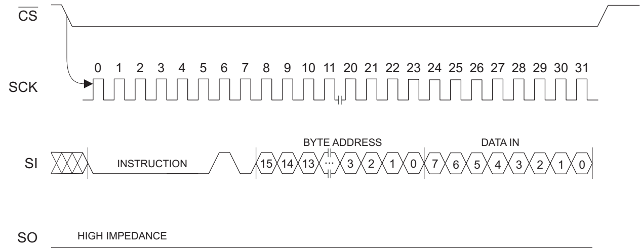
Figure 6-7. Write Timing
