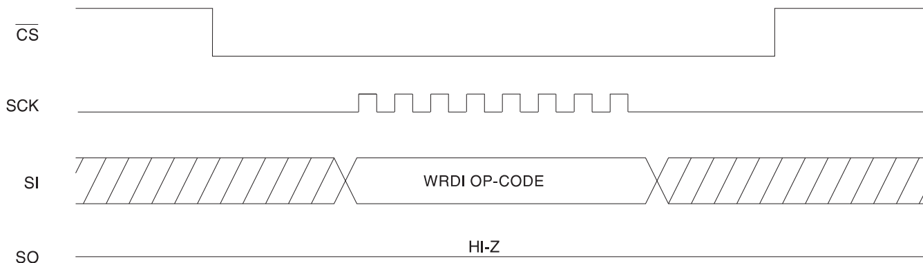
Figure 6-2. WREN Timing
