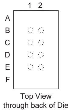
Figure 2-3. 8-ball dBGA
