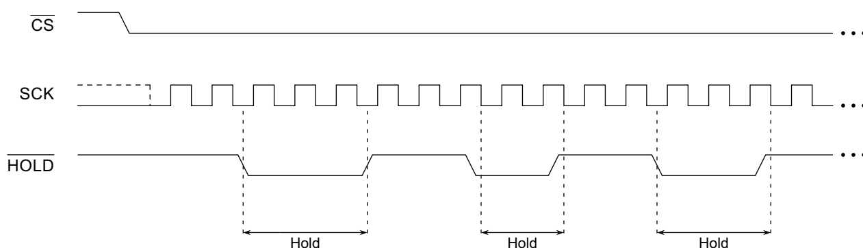
Figure 12-5. Hold Mode
