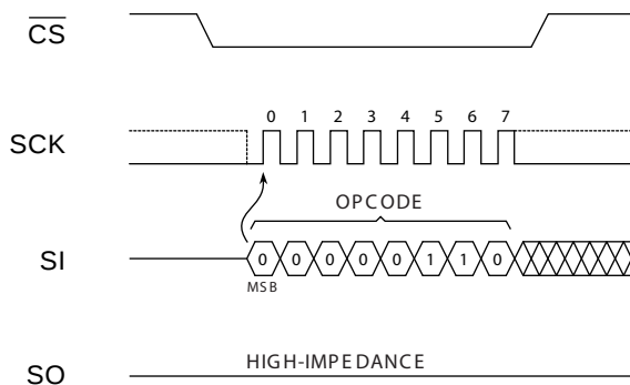
Figure 8-1. Write Enable
