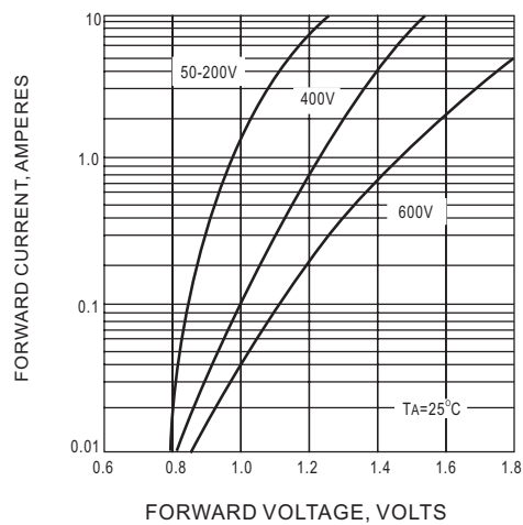
Fig.3 FORWARD CHARACTERISTICS
