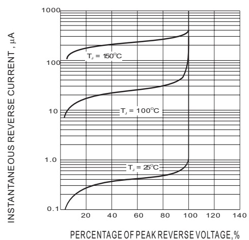
Fig.4-TYPICAL REVERSE CHARACTERISTIC
