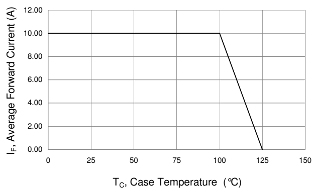
Fig.4 Forward Current Derating Curve Per Diode
