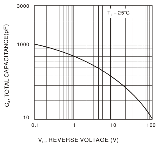
Fig.5-TYPICAL TOTAL CAPACITANCE
