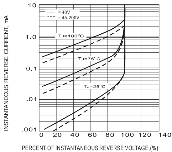
Fig.3-TYPICAL REVERSE CHARACTERISTIC
