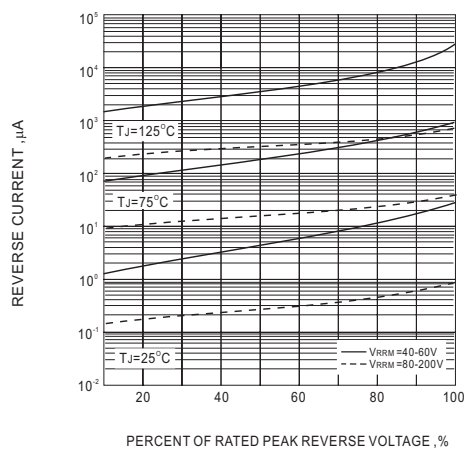
Fig.3-TYPICAL REVERSE CHARACTERISTIC
