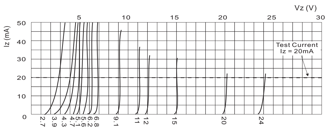
Fig.2 BREAKDOWN CHARACTERISTICS
