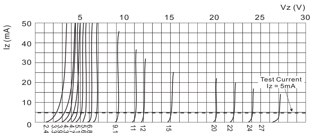
Fig.2 BREAKDOWN CHARACTERISTICS
