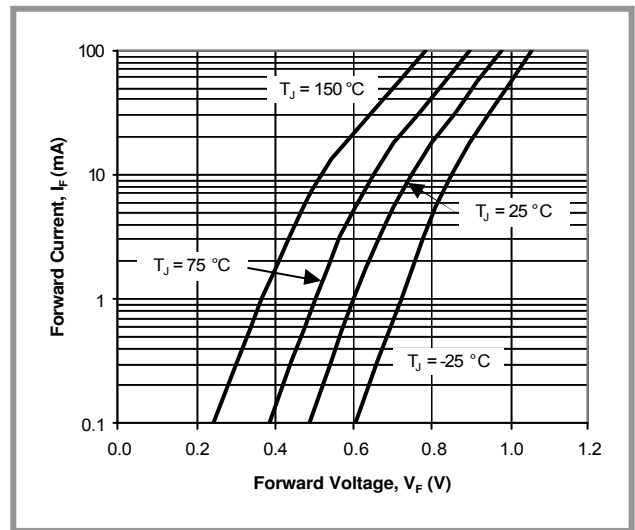
ig. 3. Forward Current vs. Forward Voltage
