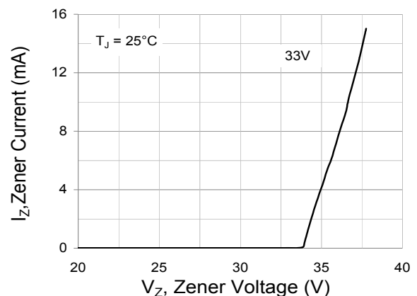
Fig.10 Typical Zener Characteristics
