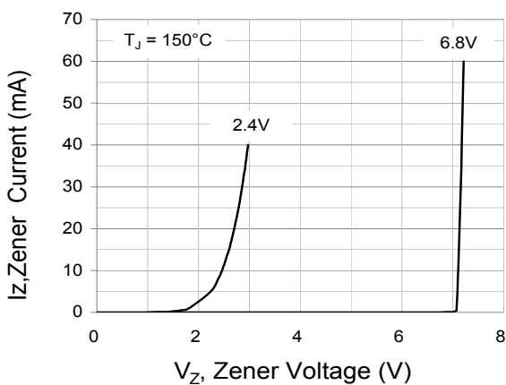
Fig.9 Typical Zener Characteristics
