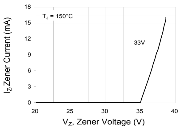
Fig.11 Typical Zener Characteristics
