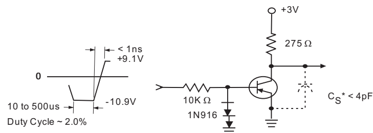
Storage and Fall Time Equivalent Test Circuit
