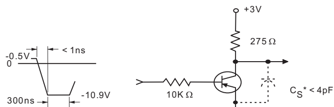
Delay and Rise Time Equivalent Test Circuit
