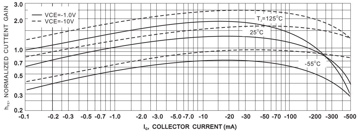
Fig.1-DC Current Gain
