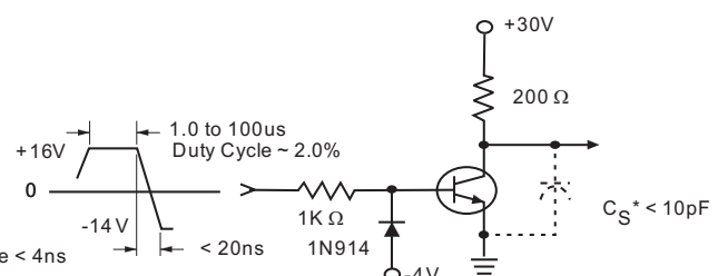
Fig. 2 Turn-Off Time
