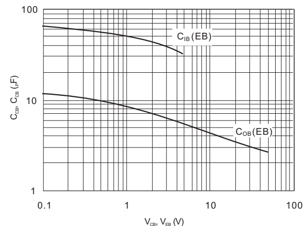
Fig.4 Typical Capacitances
