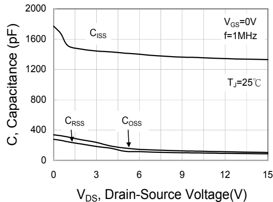
Fig.1 Capacitance Variation
