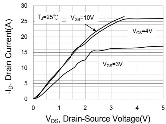
Fig.2 Drain Current VS Drain-Source Voltage
