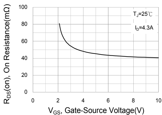
Fig.5 ON Resistance VS Gate-Source Voltage
