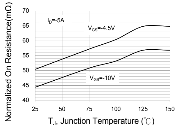
Fig.6 ON Resistance VS Junction Temperature
