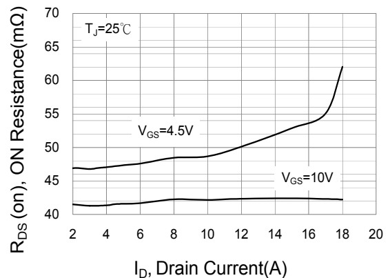
Fig.4 ON Resistance VS Drain Current
