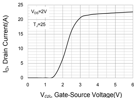
Fig.3 Drain current VS Gate Source Voltage
