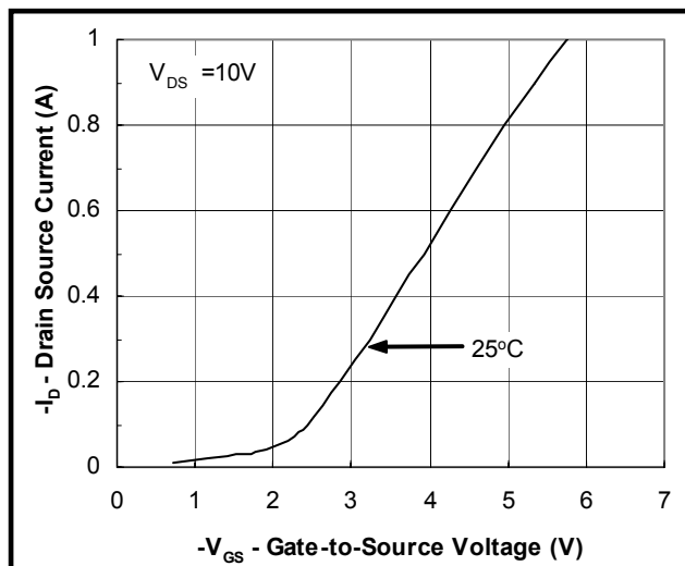
Fig. 2. Transfer Characteristics
