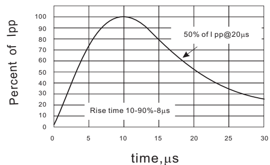
Fig.2 Pulse Waveform
