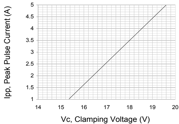
Fig.1 Typical peak clamping voltage(8/20μs)
